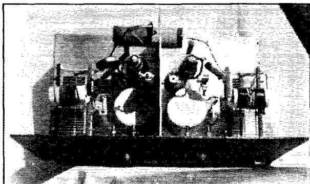
A top view of the experimental amplifier using 6F6-100's. The plate phasing coil projects through the baffle shield between the two stages. Amplifier tank coils are mounted on top of their respective condensers. The shield cans contain the grid coils.
