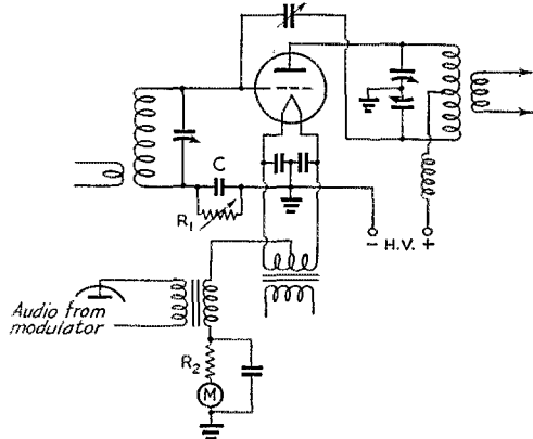
Fig. 1—The fundamental cathode-modulation circuit. Audio from the modulator unit is introduced in the cathode (center-tap) circuit of the tube or tubes being modulated. The grid-leak resistance R_1 is adjusted for proper modulation characteristics, and R_2 serves to give some original bias to the tube. Condenser C must be large enough to by-pass the modulation frequencies.
