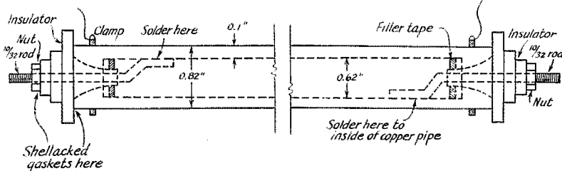
Fig. 2 — The coaxial line from the pick-up coil to the antenna is made of thin-wall electrical conduit with a piece of \frac{1}{2} -inch copper tubing running through the center. Parts of feed-through insulators support the inner conductor, and the line is made weatherproof by sealing at both ends.
