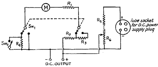
Fig. 4 — Circuit of the d.c. voltmeter.
