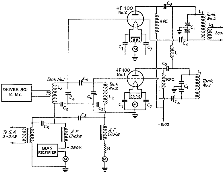
Fig. 4 — Circuit of the transmitter using HF-100's.
